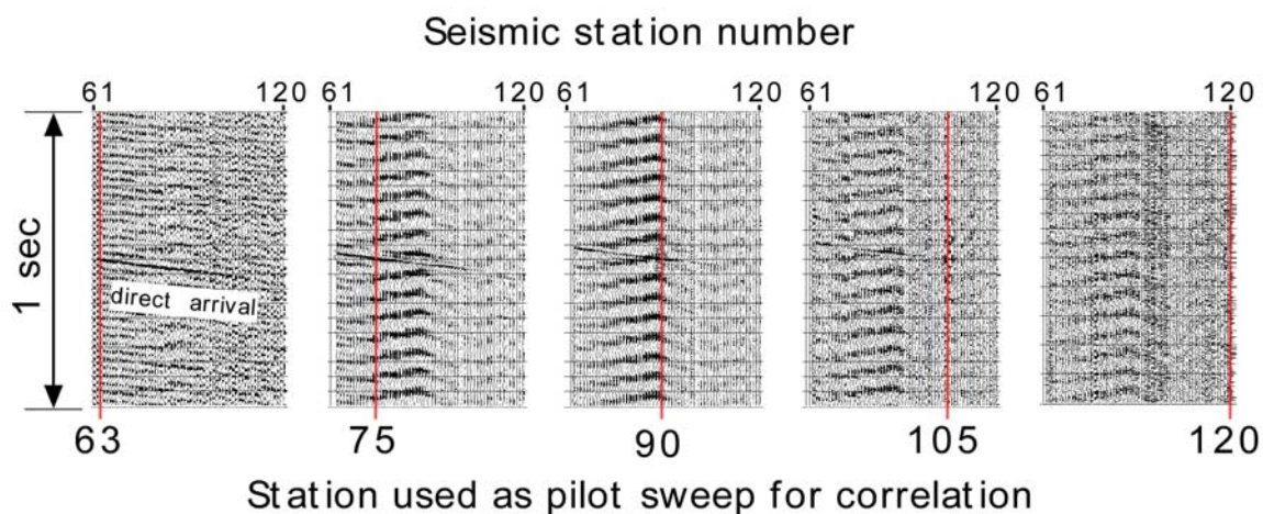
Figure 9. Examples of correlated data using various traces as the pilot trace for correlation (shown in red). The direct arrival is well developed almost regardless of the pilot trace used, although it weakens significantly at greater offset due to the critical angle of seismic energy at the coal/rock interface being approached and the increasingly emergent wave at the vertical geophone at greater offsets. The distinct concave downward oscillatory signal seen in some raw data (Figure 6) is well developed in most correlated records when using pilot traces in the 70-90 range, as seen above.
